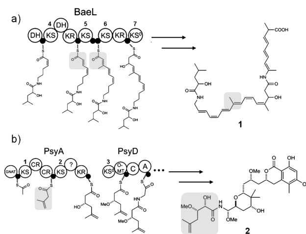
Scheme 1. Partial proposed biosynthetic schemes for a) bacillaene 1 and b) psymberin 2. KS = ketosynthase; KS 0 = non-elongating ketosynthase; KR = ketoreductase; DH = dehydratase; CR = crotonase; O-MT = O-methyl transferase; C = NRPS condensation domain; A = NRPS adenylation; GNAT = acetyl-loading AT; ACP domains (●). The sequential KS numbering is denoted above the KS domains, and relevant carbon-branched regions of the intermediates are highlighted in gray.
